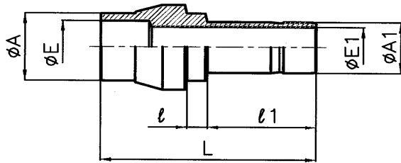
TYPE-REDUCER
