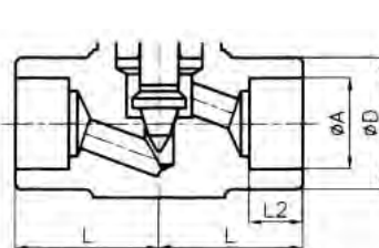
PSW : Connection
