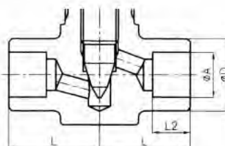
PSW : Connection
