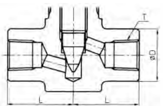
RF : Connection
